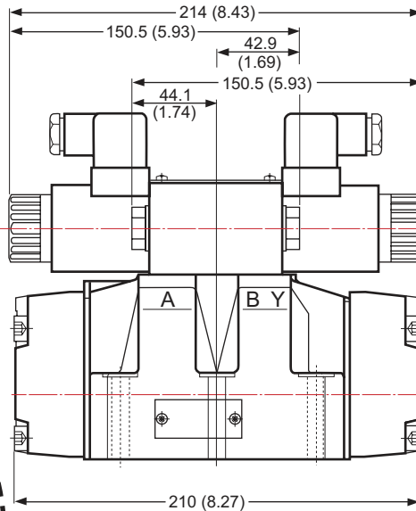
External Pilot
