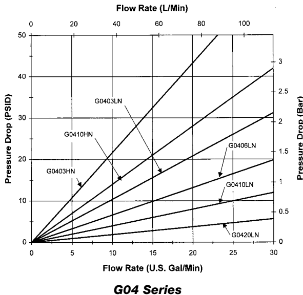
Average Pressure Drop Through Clean Element With 150 SUS Oil At 100° F (32 cSt at 40° C)
